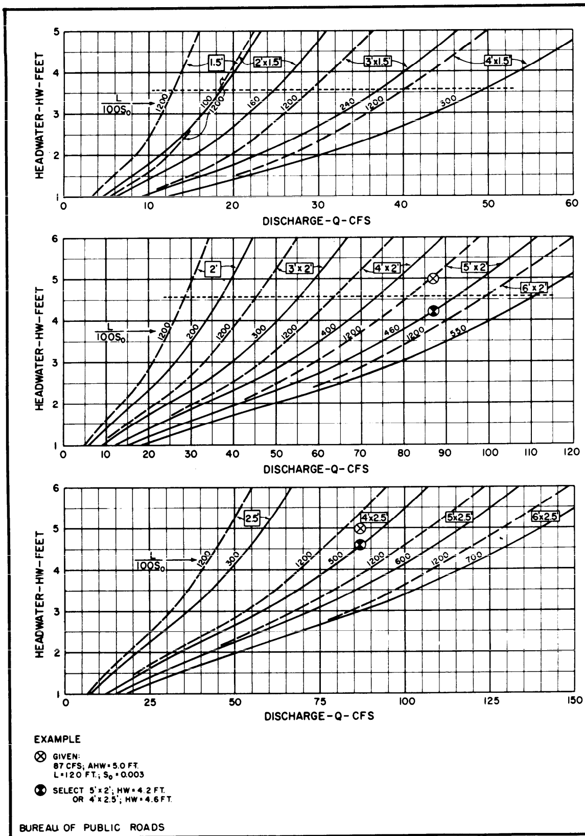
Figure B-41. Culvert capacity rectangular concrete box 80° to 75° wingwall flare 1.5', 2.0' and 2.5' heights.
