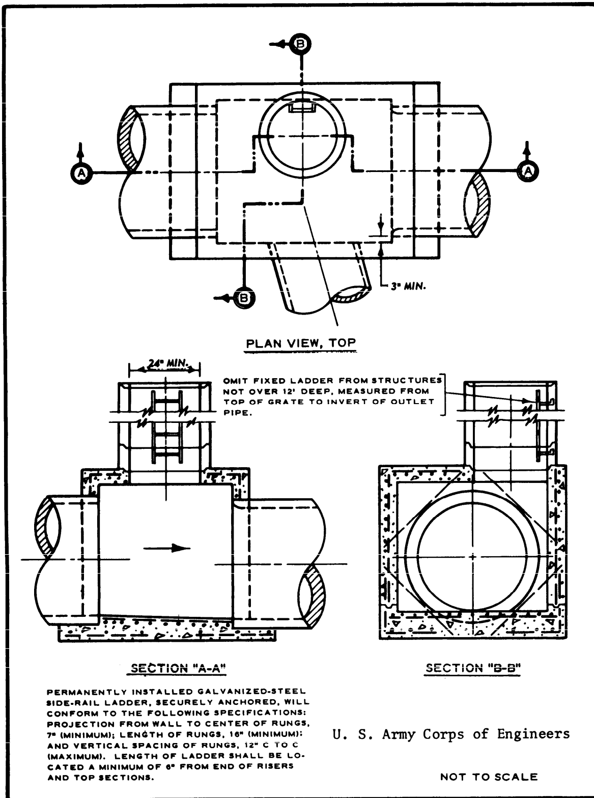
Figure 4-3. Junction details for large pipes.
