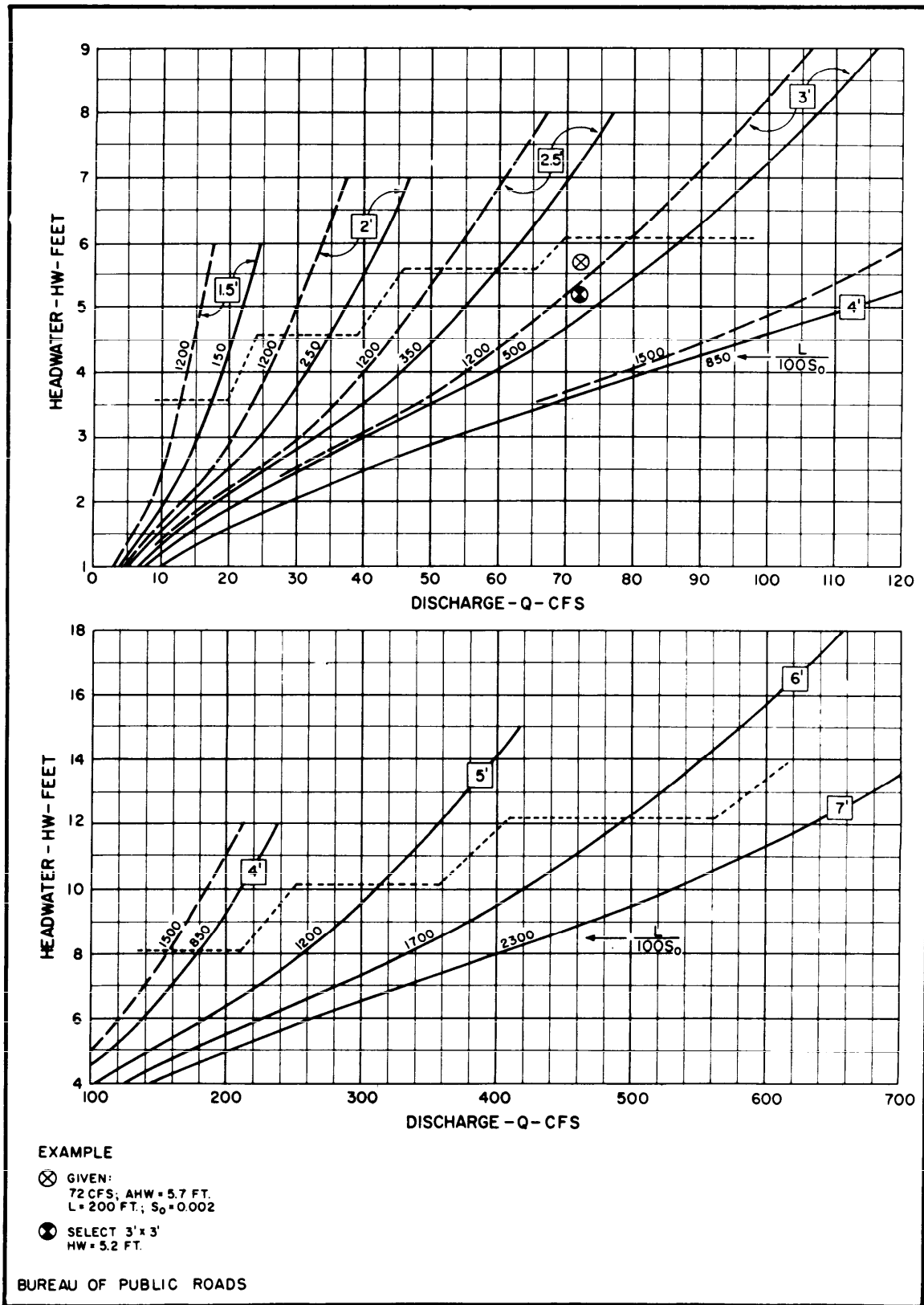
Figure B-36. Culvert capacity square concrete box 90° and 15° wingwall flare 1.5' x 1.5' to 7' x 7'.
