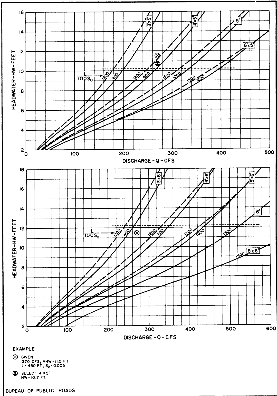
Figure B-48. Culvert capacity rectangular concrete box 30° to 75° wingwall flare 5' and 6' heights.
