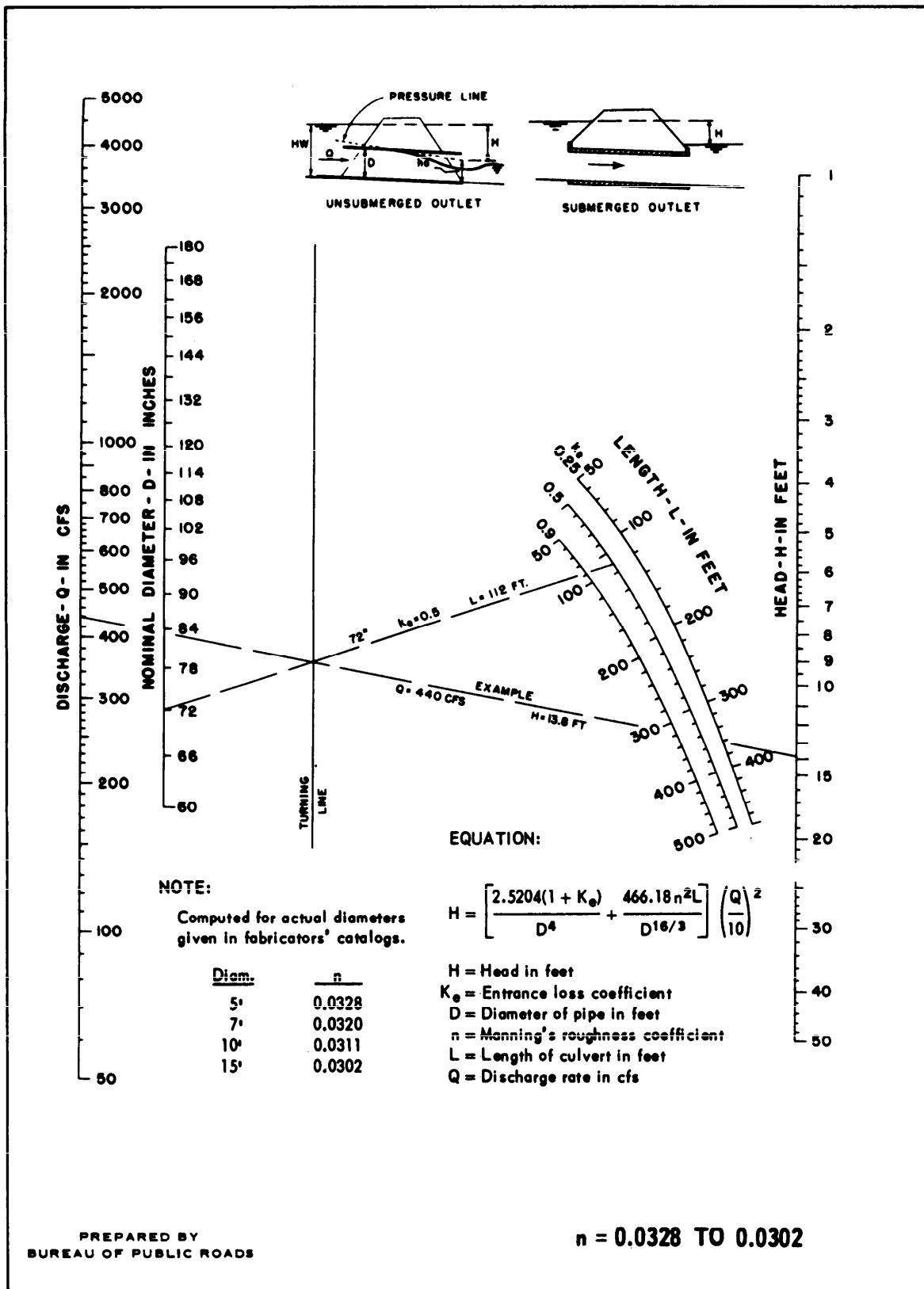
Figure B-14. Head for circular pipe culverts flowing full, n = 0.0328 to 0.0302 .
