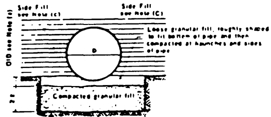
(C) FOUNDATION STABILIZATION FOR SMALL DIAMETER STRUCTURES
