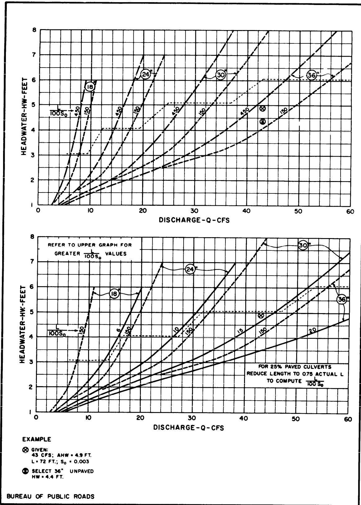
Figure B-30. Culvert capacity standard circular corrugations metal headwall entrance 18" to 36".
