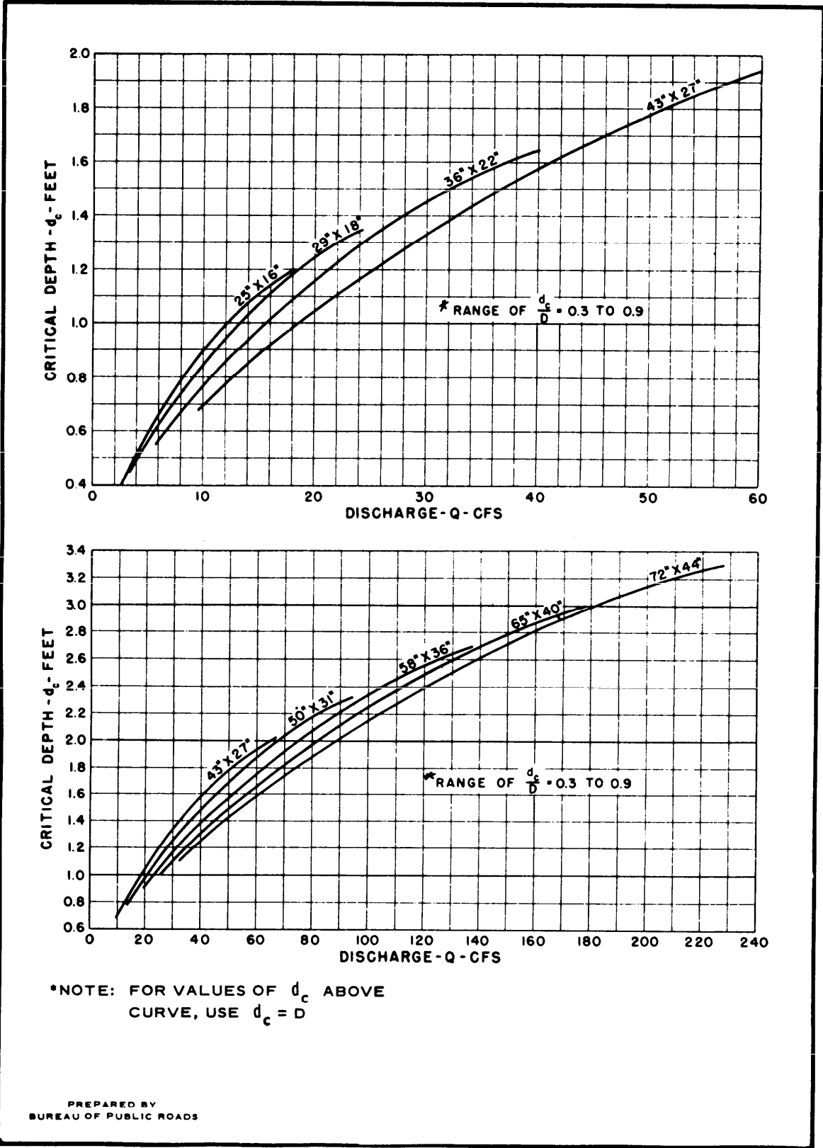
Figure B-23. Standard corrugated metal pipe-arch critical depth.
