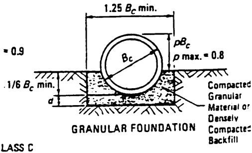
Depth of Bedding Material Below Pipe
