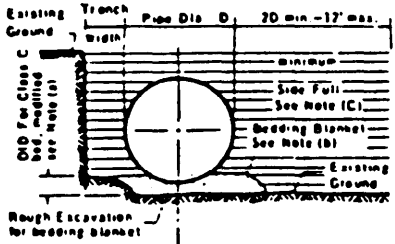
(A) PIPE INSTALLATION AND BEDDING
