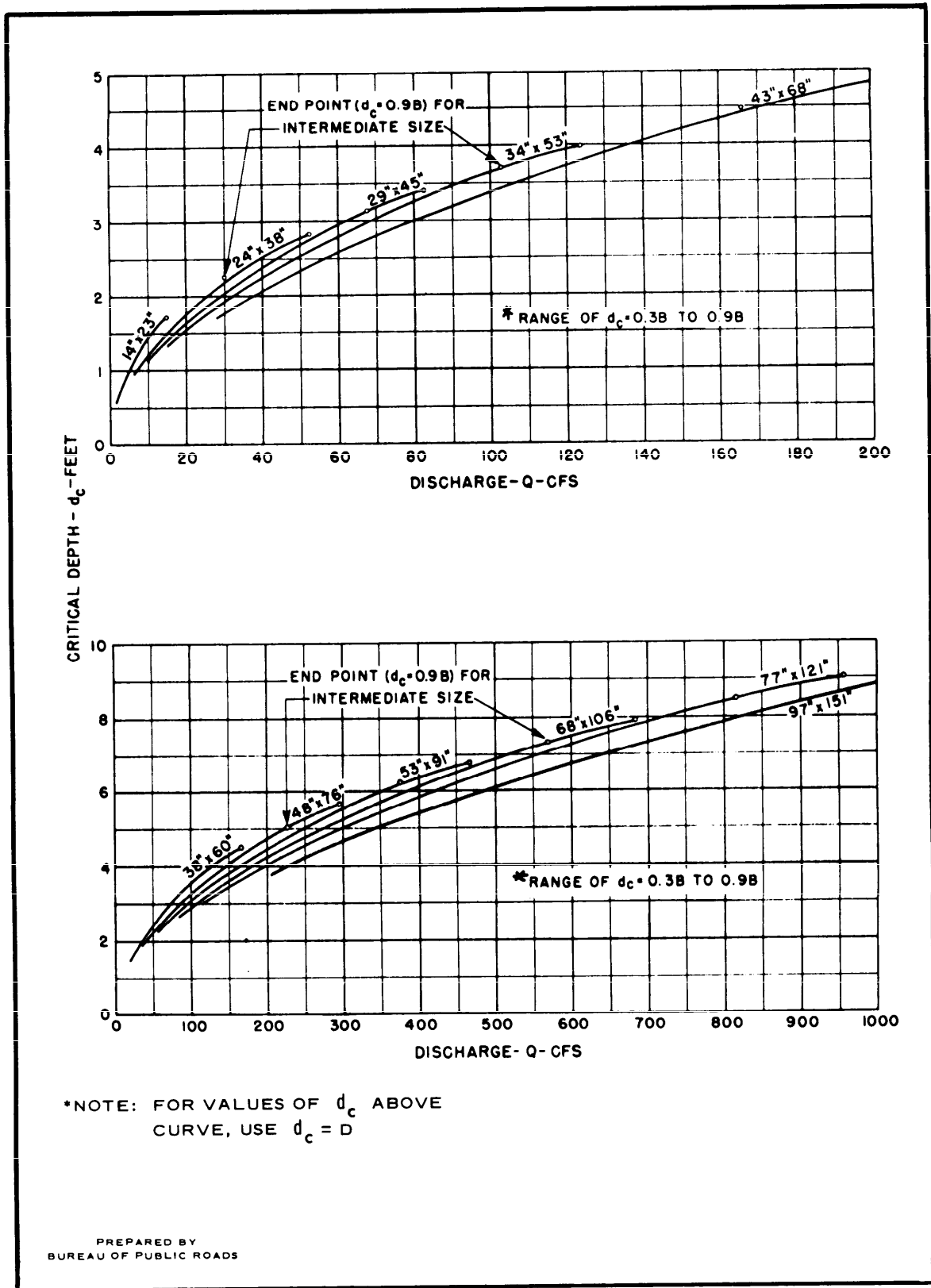
Figure B-22. Oval concrete pipe long axis vertical critical depth.
