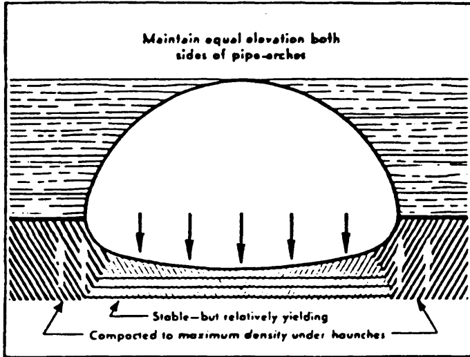
Recommended backfilling practice for pipe-arch.
