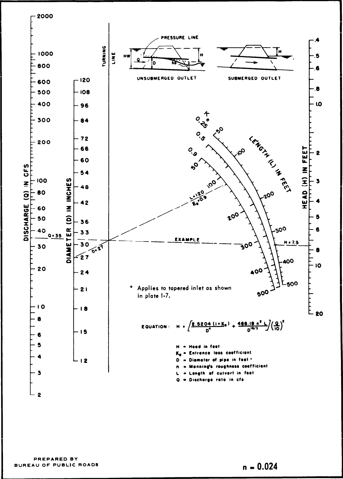
Figure B-18. Head for circular pipe culverts flowing full, n = 0.024.
