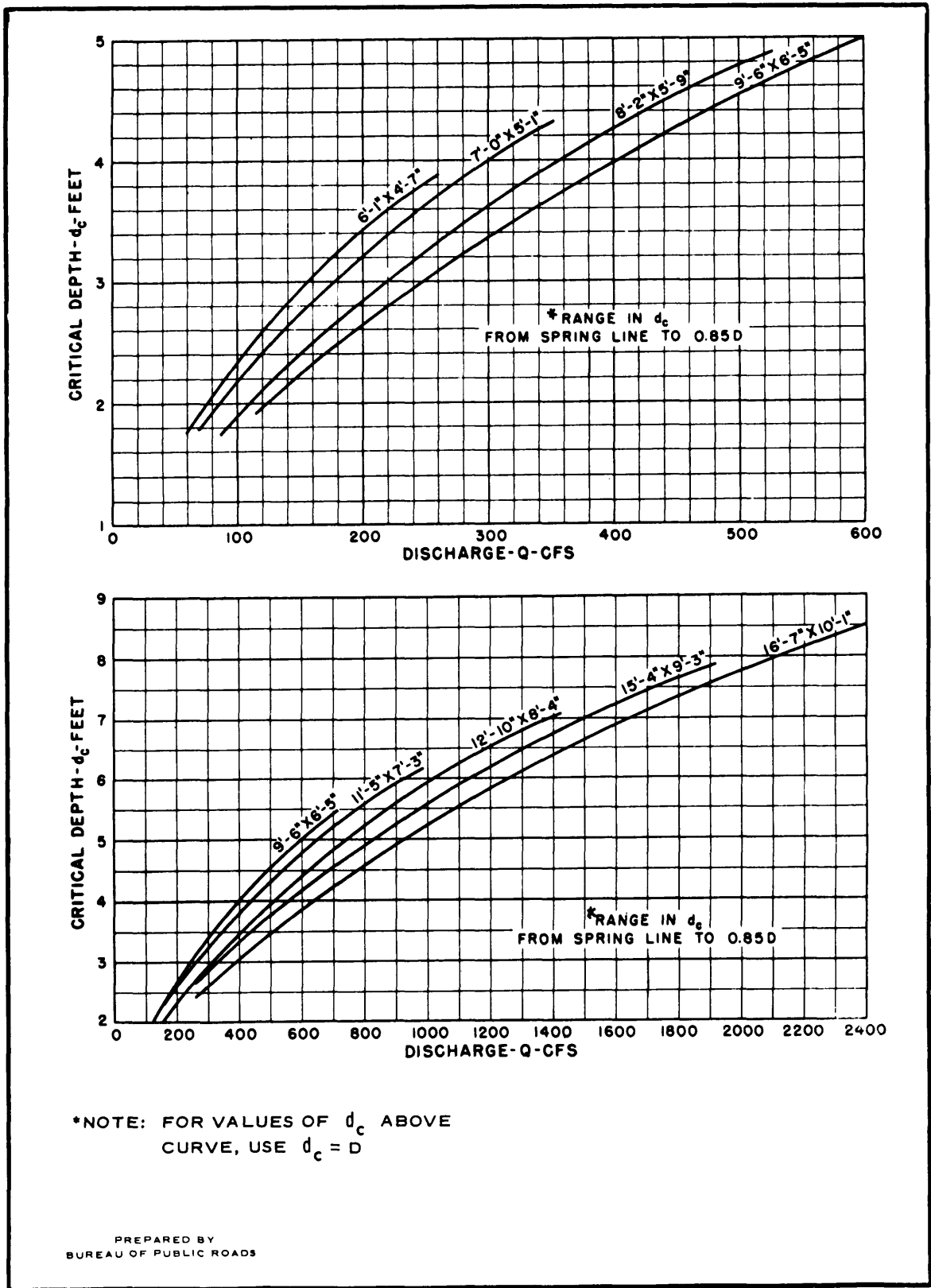
Figure B-24. Structural plate pipe-arch critical depth.
