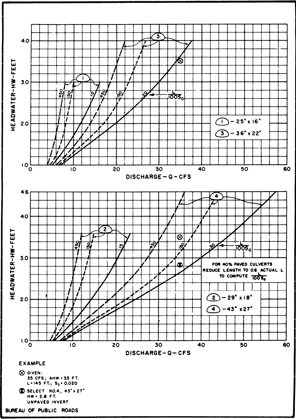
Figure B-34. Culvert capacity standard corrugations metal pipe-arch headwall entrance 25" x 18" to 43" x 27".
