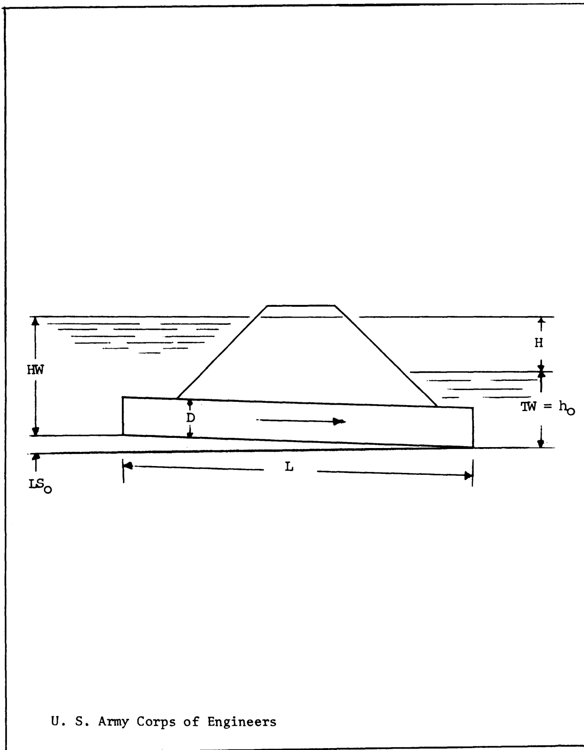
Figure B-18. Tailwater elevation at or above top of culvert.
