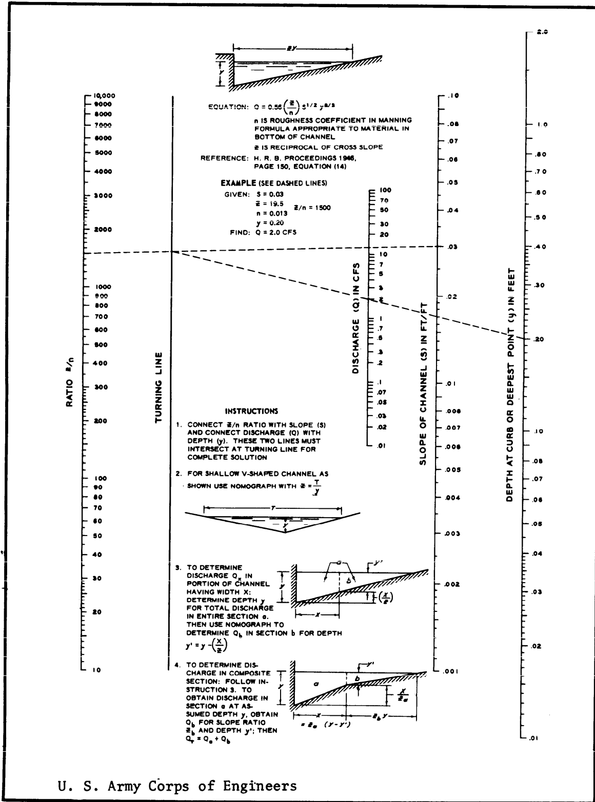
Figure 3-2. Nomograph for flow in triangular channels.
