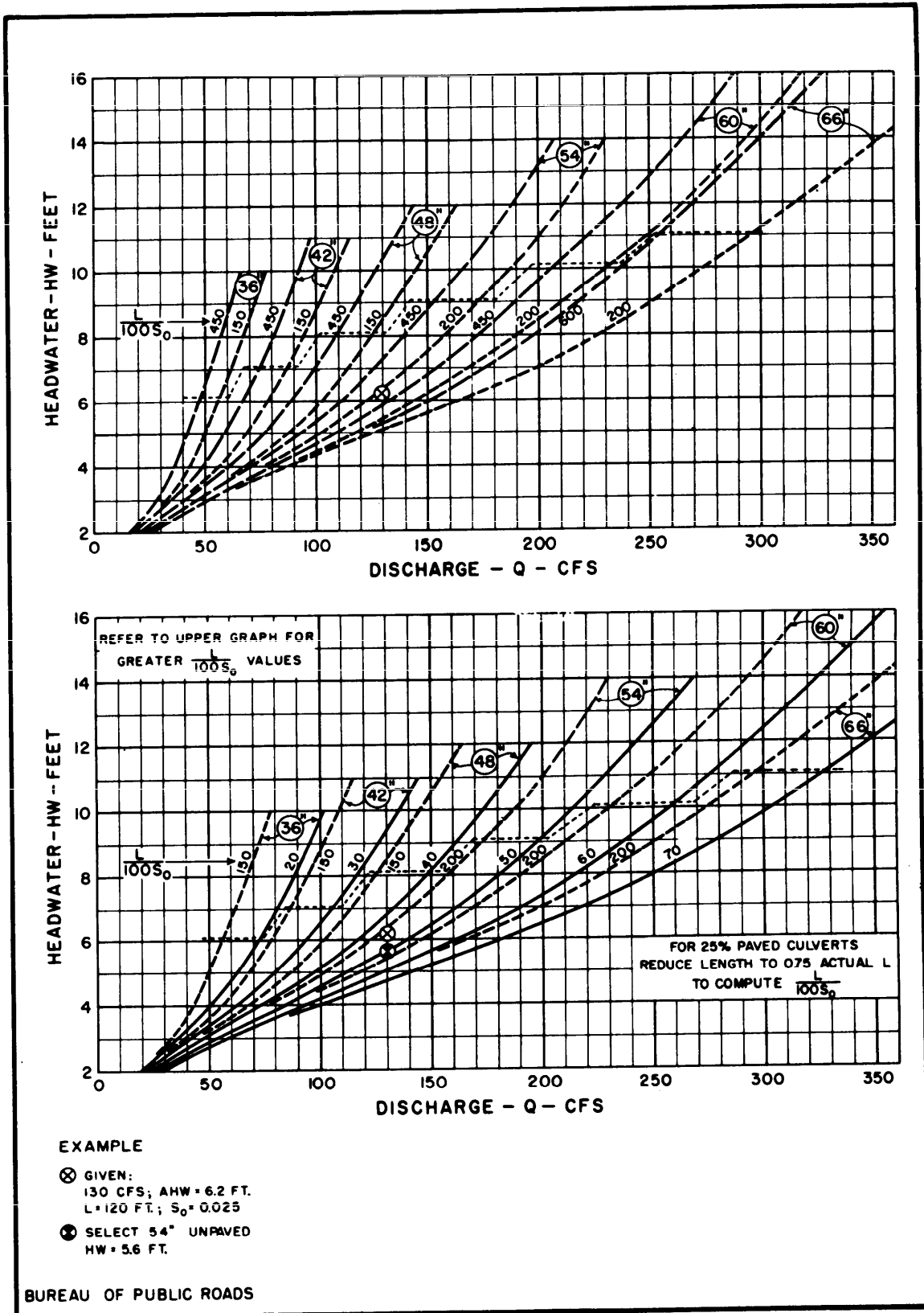
Figure B-31. Culvert capacity standard circular corrugations metal headwall entrance 36" to 66".
