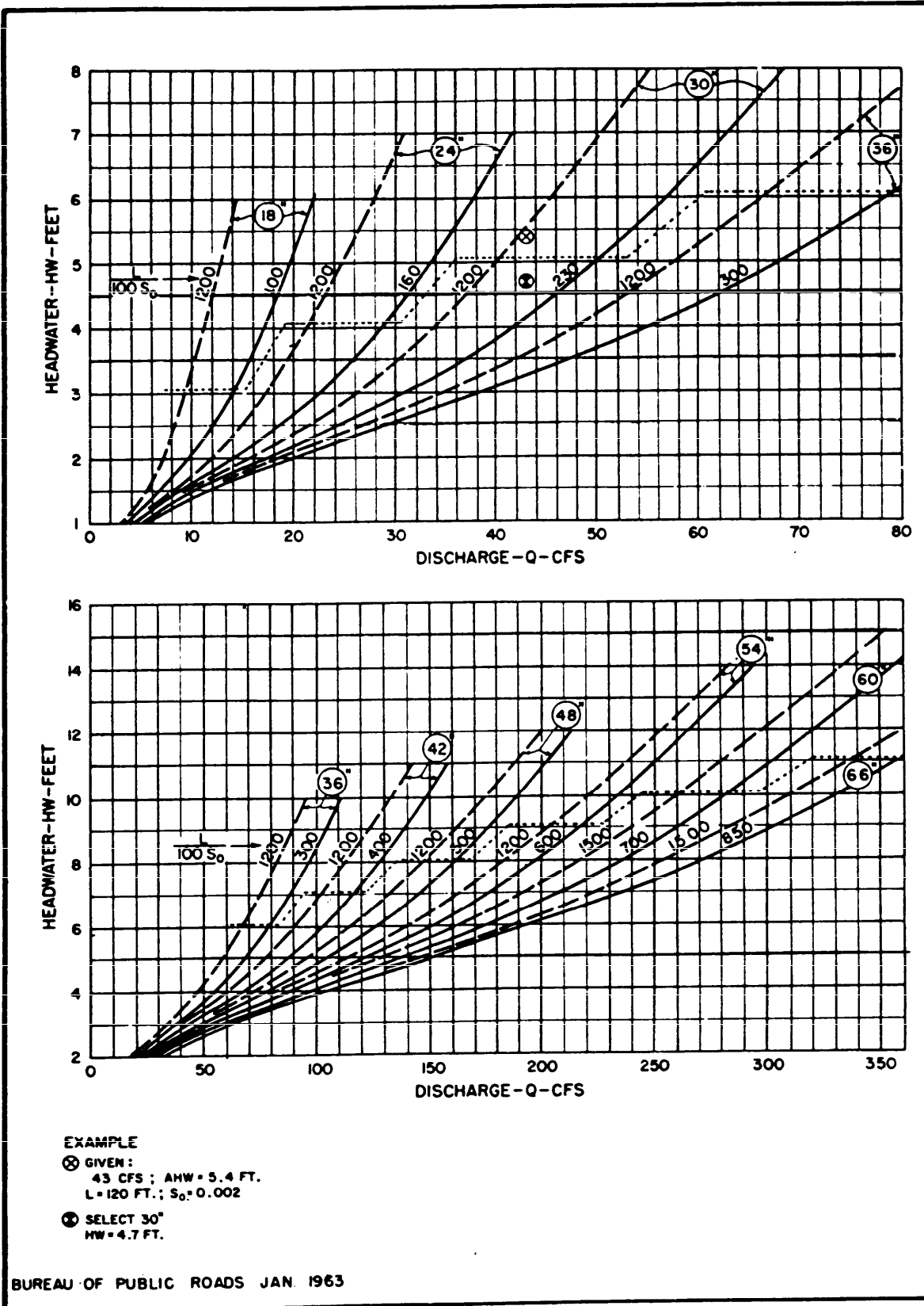
Figure B-26. Culvert capacity circular concrete pipe groove-edged entrance 18" to 66".
